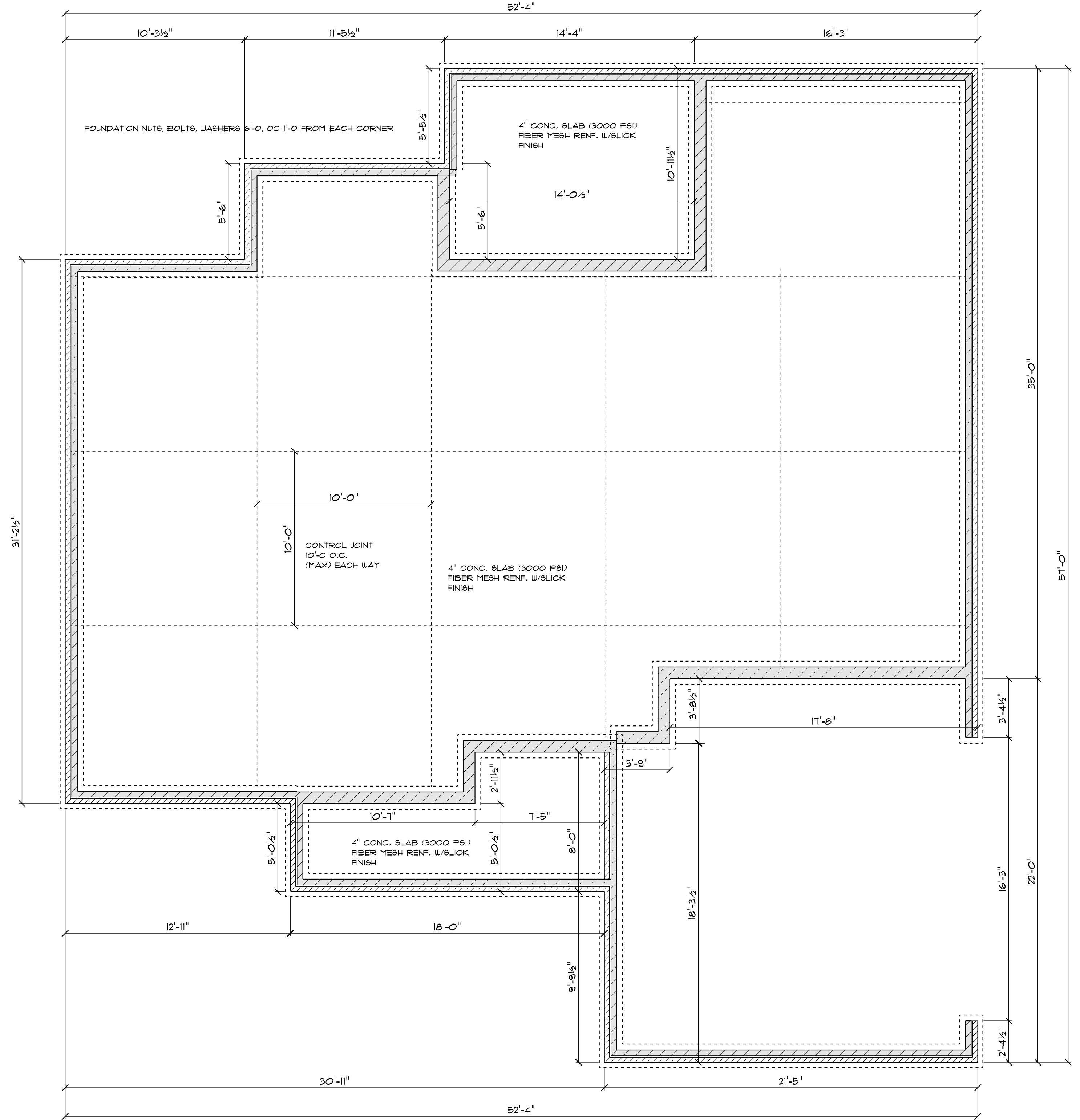
FOUNDATION PLAN SCALE: 1" = 1/4"
